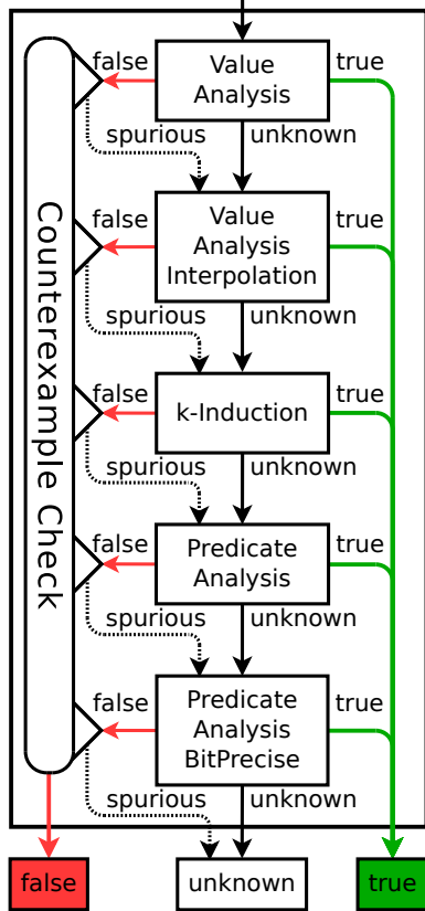
Fig. 1. Sequential combination to verify reachability properties
